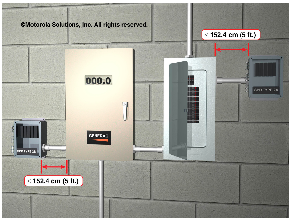
Figure 7-1 Minimum AC Surge Protection Installation Complement for a Typical Communications Site
