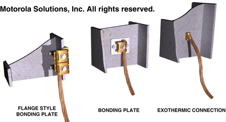
Figure 4-97 Acceptable Structural Building Steel Bonding Connections
