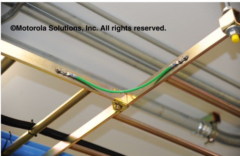
Figure 5-97 Example of Bonding Jumper Installed on Cable Tray System
