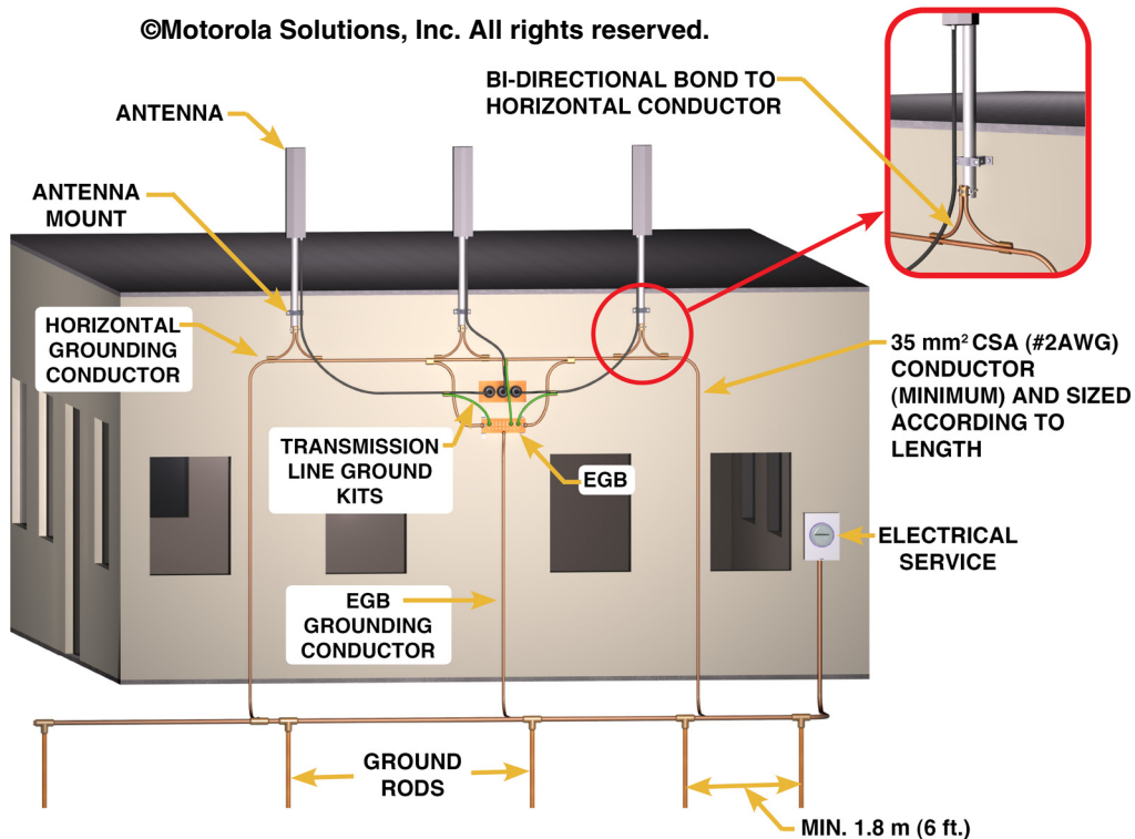
Figure 4-100 Grounding of Multiple Side-Mounted Antennas
