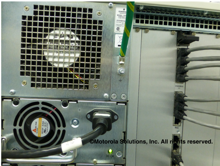
Figure 5-90 Example of Equipment Bonding - Trunking Controller
