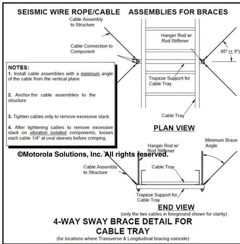
Figure 9-11 Brace Detail for Cable Tray
