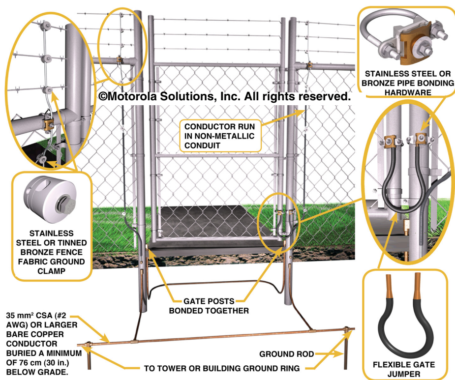
Figure 4-87 Example of Gate Bonding
