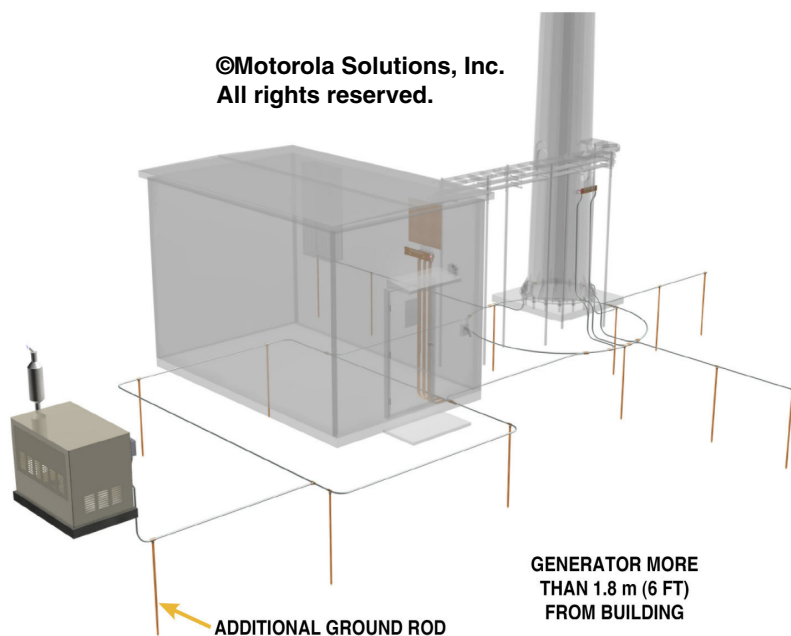
Figure 4-75 Generator Grounding: More than 1.8 m (6 ft) from Building
