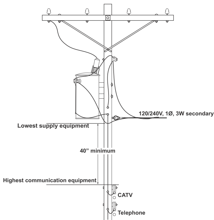
Figure 9-62 Vertical Clearance Between Communication Equipment and Non-Current-Carrying Parts (Secondary Below Bottom of Grounded Case)
