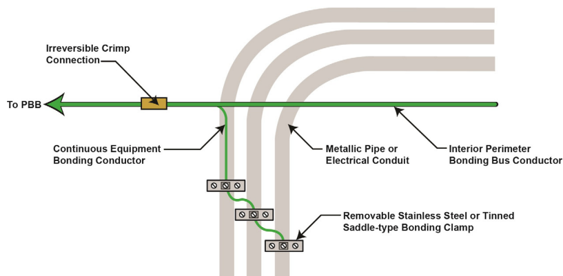
Figure 5-99 Bonding Method for Metallic Pipe or Conduit
