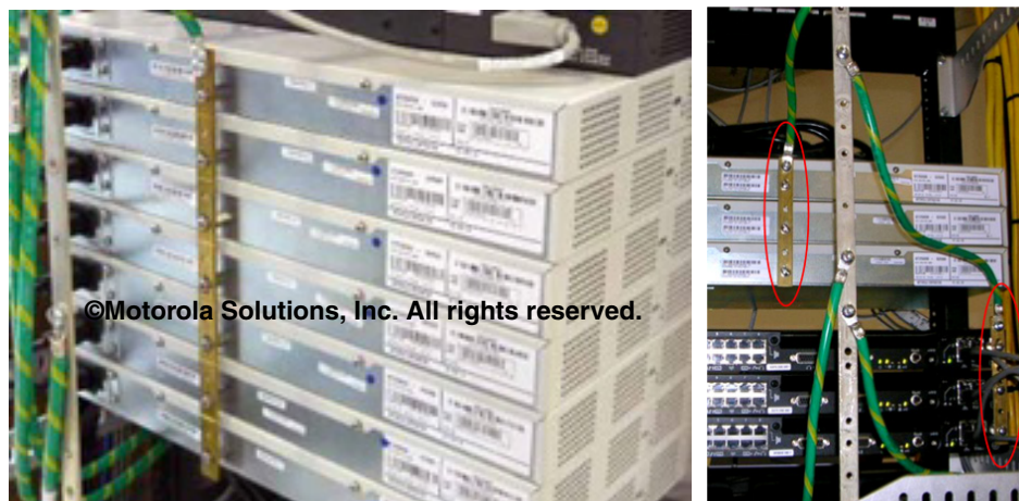
Figure 5-33 Typical Network-Equipment Bonding Bar Mounting Locations
