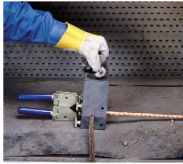
STEP 2: Close handle clamp and lock mold. Insert disk into mold.
