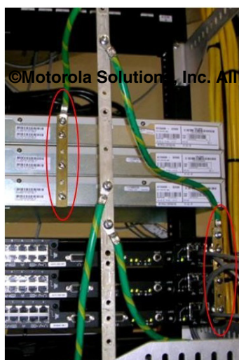
Figure 5-32 Rack with Two Network-Equipment Bonding Bars
