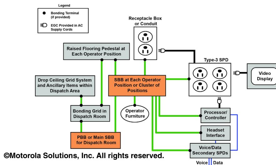
Figure 5-141 Example of Network Operator Position Bonding
