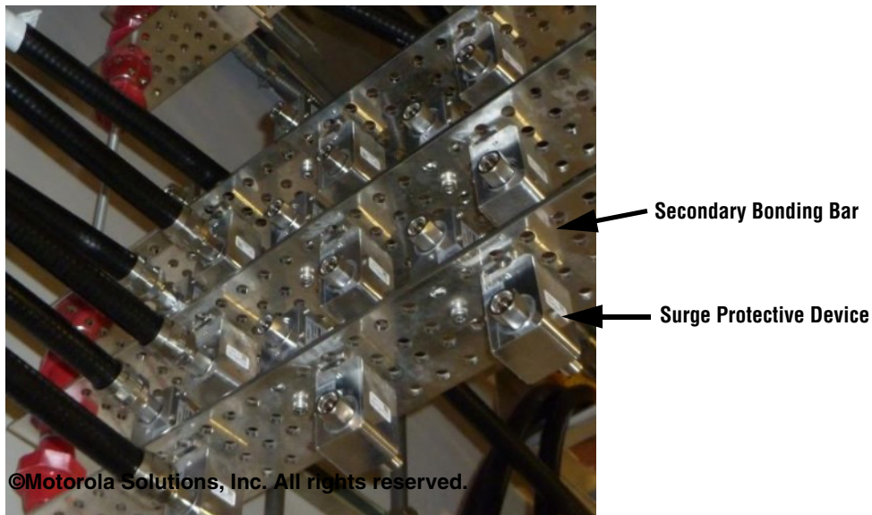
Figure 7-30 Example of RF Surge Protective Device Entry Trapeze Assembly
