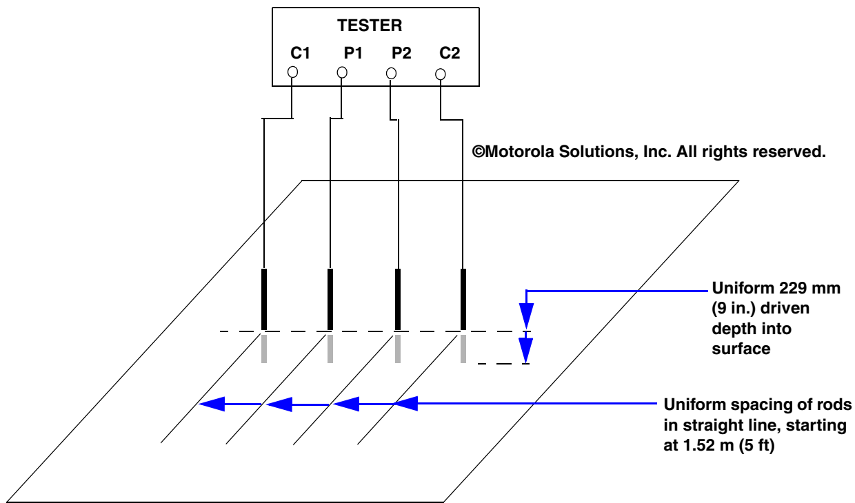
Figure B-4 Rod Arrangement and Spacing
