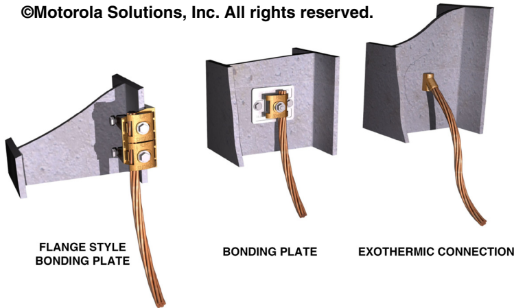
Figure 5-69 Examples of Acceptable Structural Building Steel Bonding Connections
