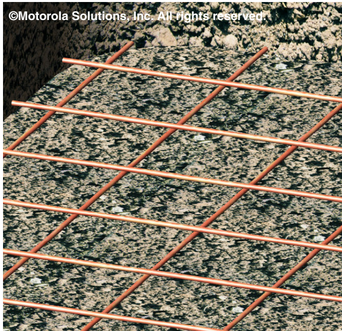
Figure 4-32 Wire Mesh Close-up View (Ground Cover Not Shown)
