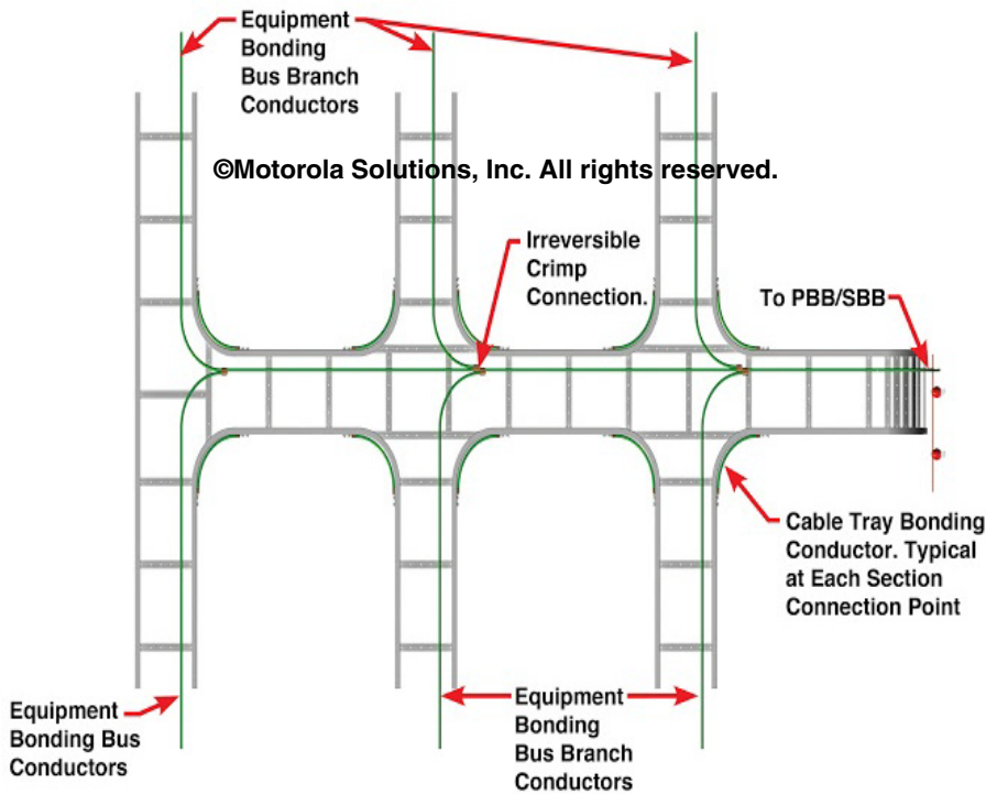
Figure 5-127 Example of Equipment Bonding Bus Conductors
