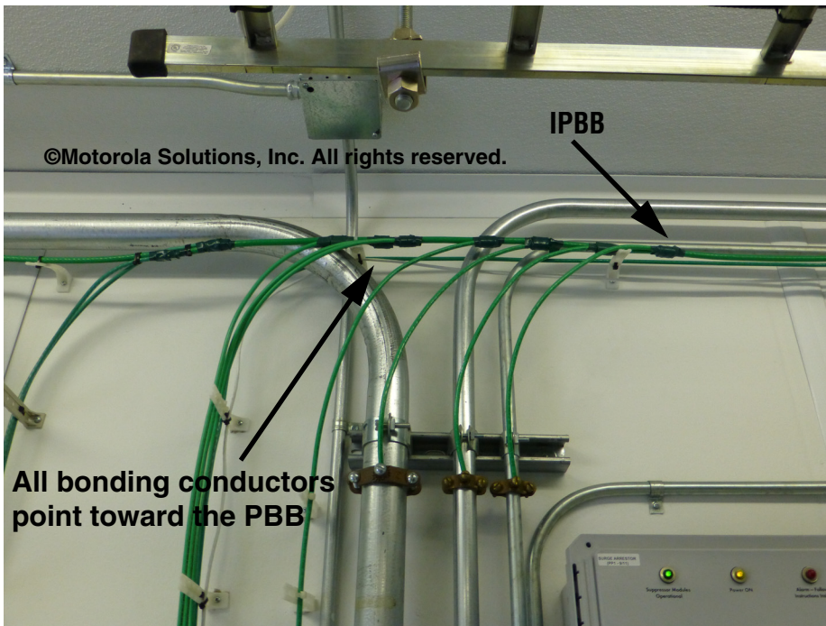
Figure 5-75 Bonding to the Internal Perimeter Bonding Bus (IPBB) Conductor
