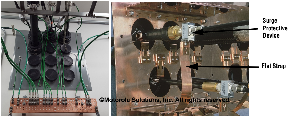
Figure 7-32 Examples of RF SPD Bonding - Round Conductor and Flat Strap (Preferred)
