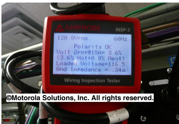
Figure 6-9 Example of Receptacle Tester
