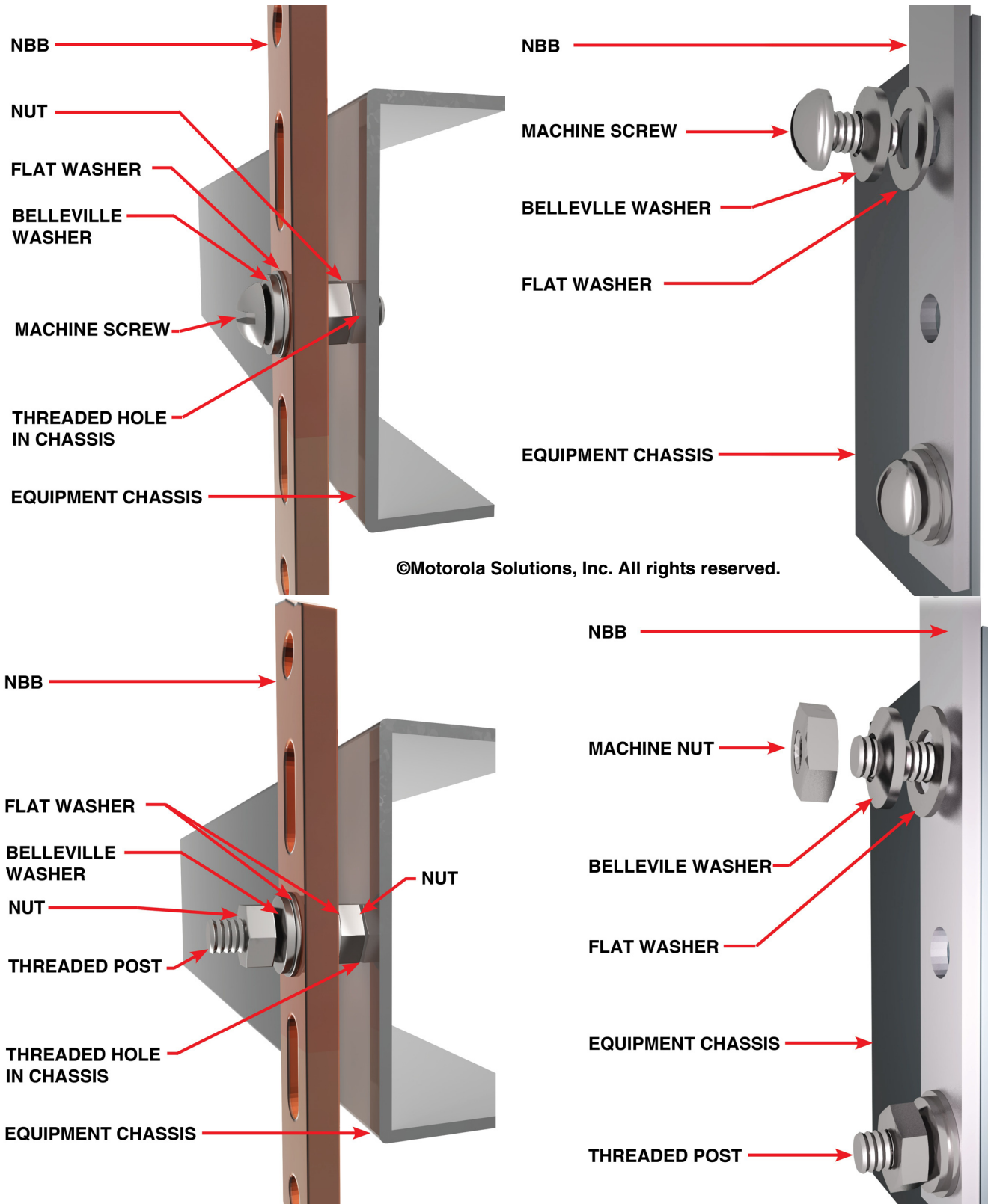
Figure 5-35 Examples of Bonding a Network-Event Bonding Bar to an Equipment Chassis with Belleville Washers
