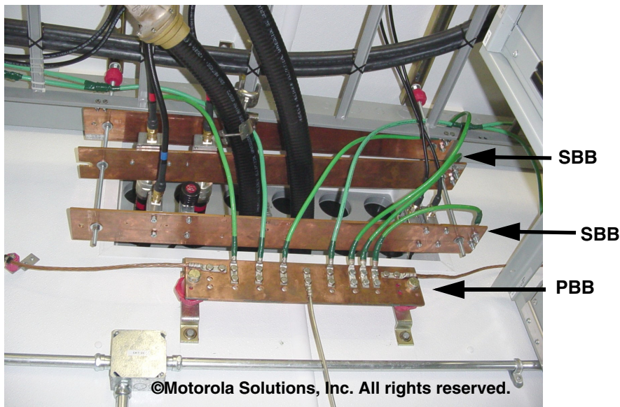
Figure 5-22 Ceiling Supported Secondary Bonding Bars at a Ceiling Level Communications Cable Entry
