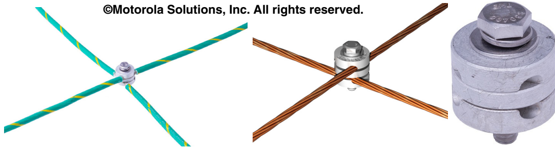
Figure 5-61 Examples of Bonding Grid Listed Clamps
