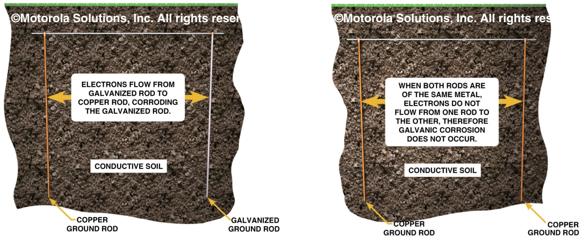
Figure 4-49 Installations With and Without Galvanic Corrosion
