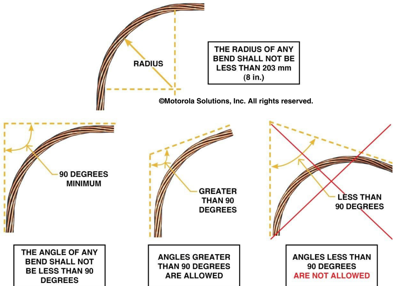
Figure 5-38 Minimum Conductor Bending Radius
