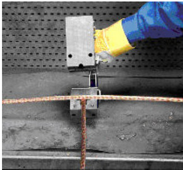
STEP 1: Clean and dry conductors and mold. insert conductors into mold.
