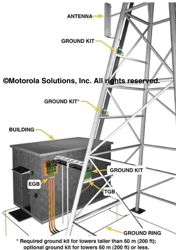
Figure 4-82 Location of Transmission Line Grounding Kits
