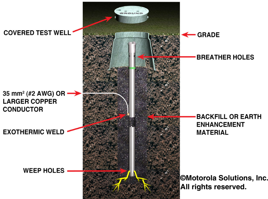
Figure 4-17 Electrolytic Ground Rod: Straight
