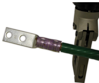
Figure 5-68 Irreversible Compression Connector and Typical Crimping Tool
