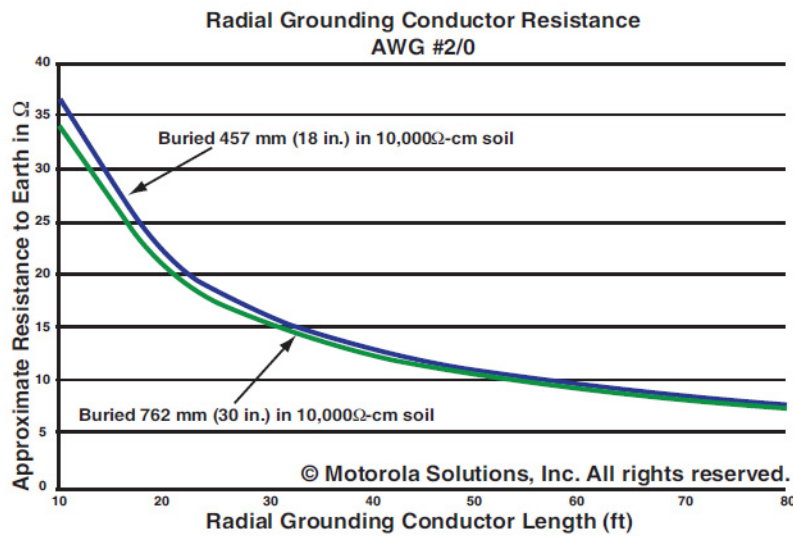
Figure 4-29 Resistance Characteristics of a Radial Grounding Conductor
