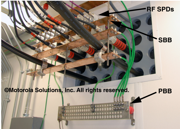
Figure 7-31 Example of RF Surge Protective Devices Bonding and Grounding Directly to Secondary Bonding Bars
