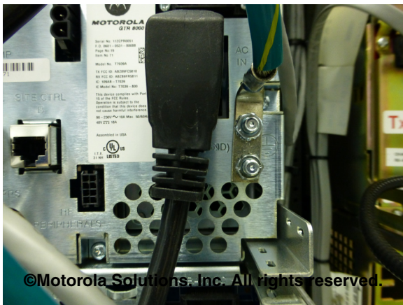
Figure 5-91 Example of Equipment Bonding - Base Station/Repeater
