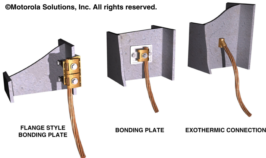
Figure 5-132 Examples of Acceptable Structural Building Steel Bonding Connections
