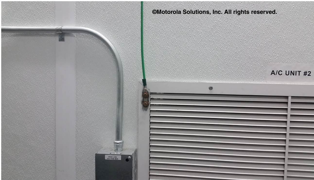
Figure 5-101 Example of HVAC Grill Bonding
