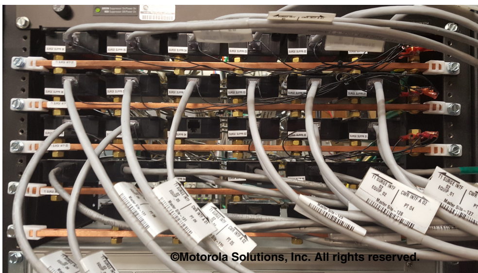
Figure 5-120 Example of Multiple Line Secondary Surge Protective Device
