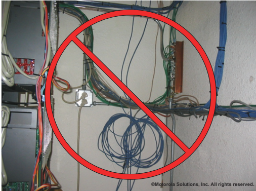
Figure 9-17 Example of Incorrectly Secured Cabling
