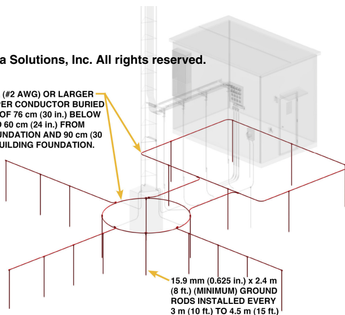
Figure 4-25 Example of Building and Tower Ground Ring With Radials
