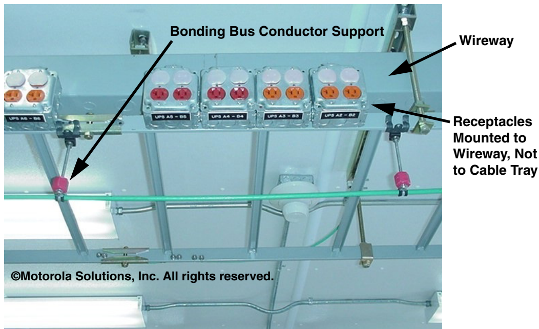
Figure 5-40 Supporting Bonding Bus Conductor on Outside of Cable Tray
