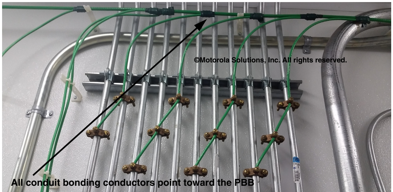
Figure 5-100 Example of Bonding Conduit to Internal Perimeter Bonding Bus
