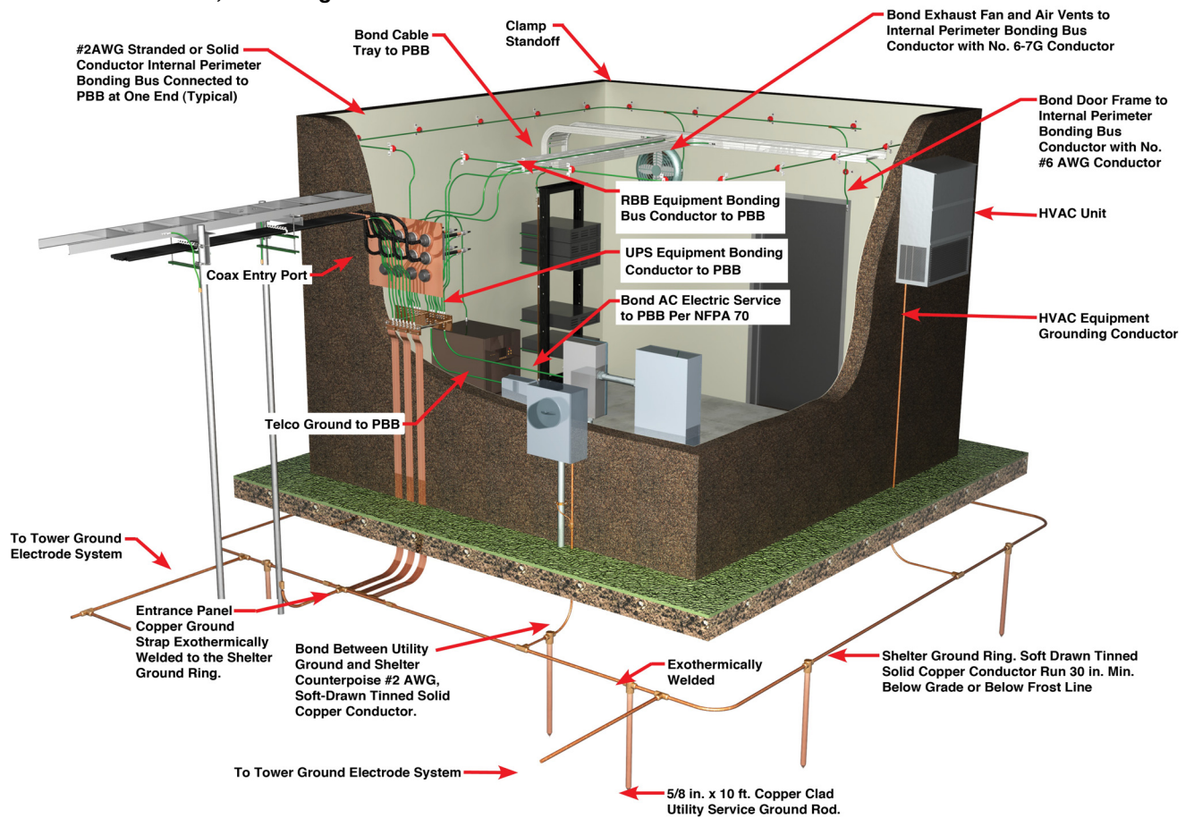
Figure 5-4 Example of Internal Bonding and Grounding System for Typical Dedicated Communications Shelter
