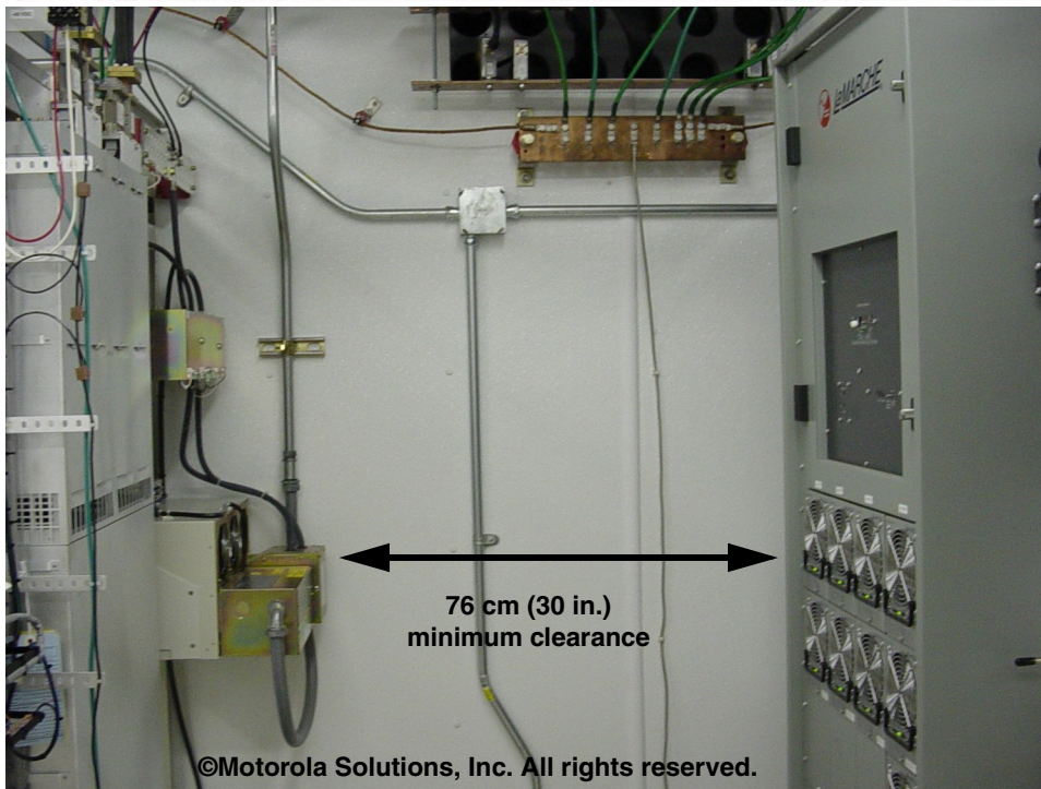
Figure 9-4 Examples of Aisle Width
