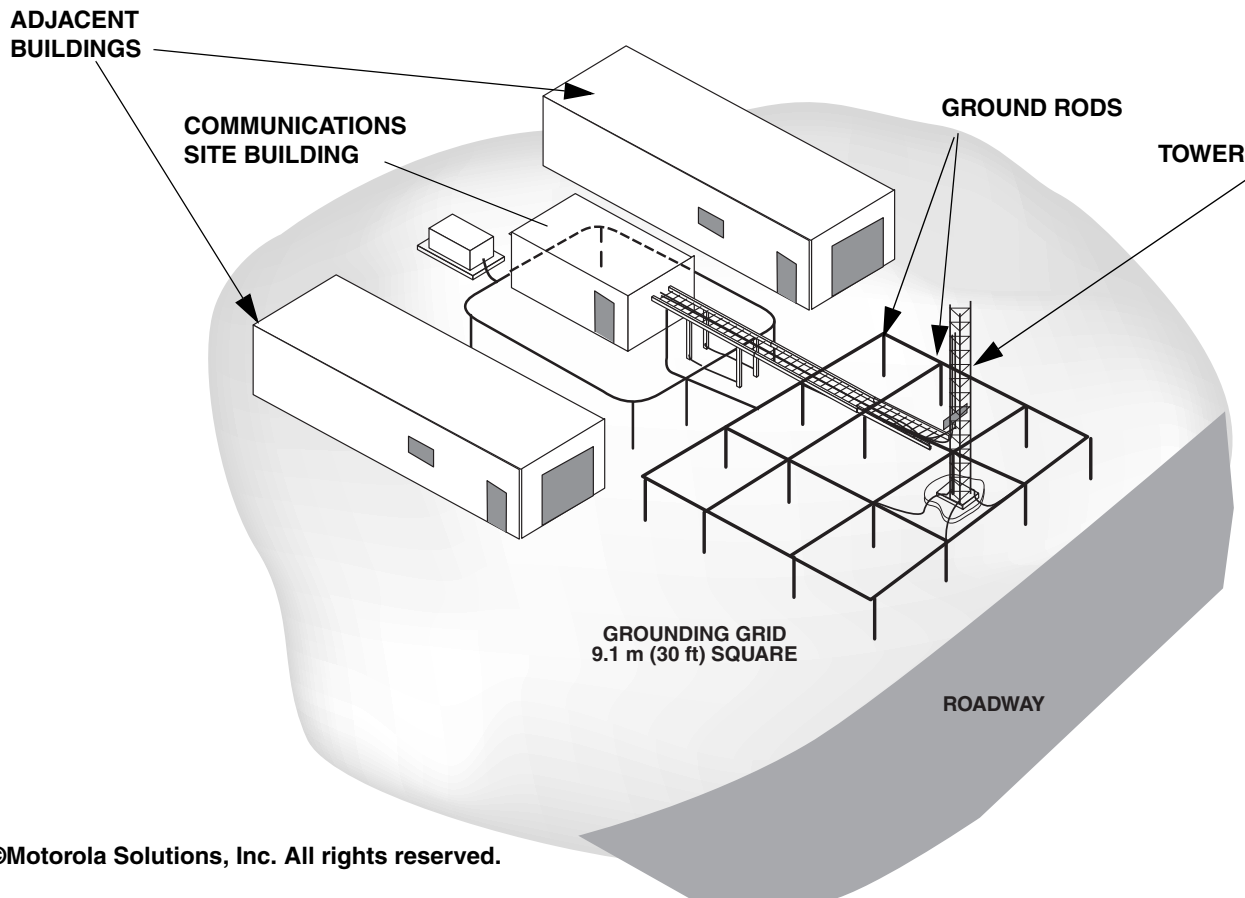
Figure B-15 Example of Multiple Ground Rod Grid Configuration
