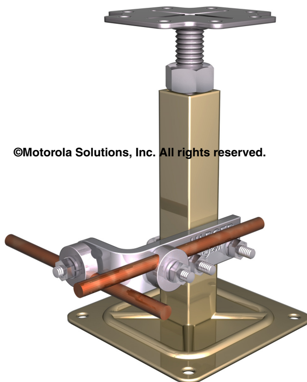
Figure 5-113 Bonding Conductors Suspended on Raised Flooring Pedestals
