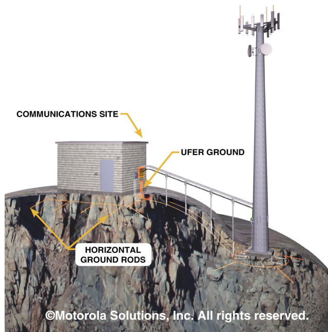
Figure 4-118 Installation of Horizontal Ground Rods in Shallow Topsoil Conditions
