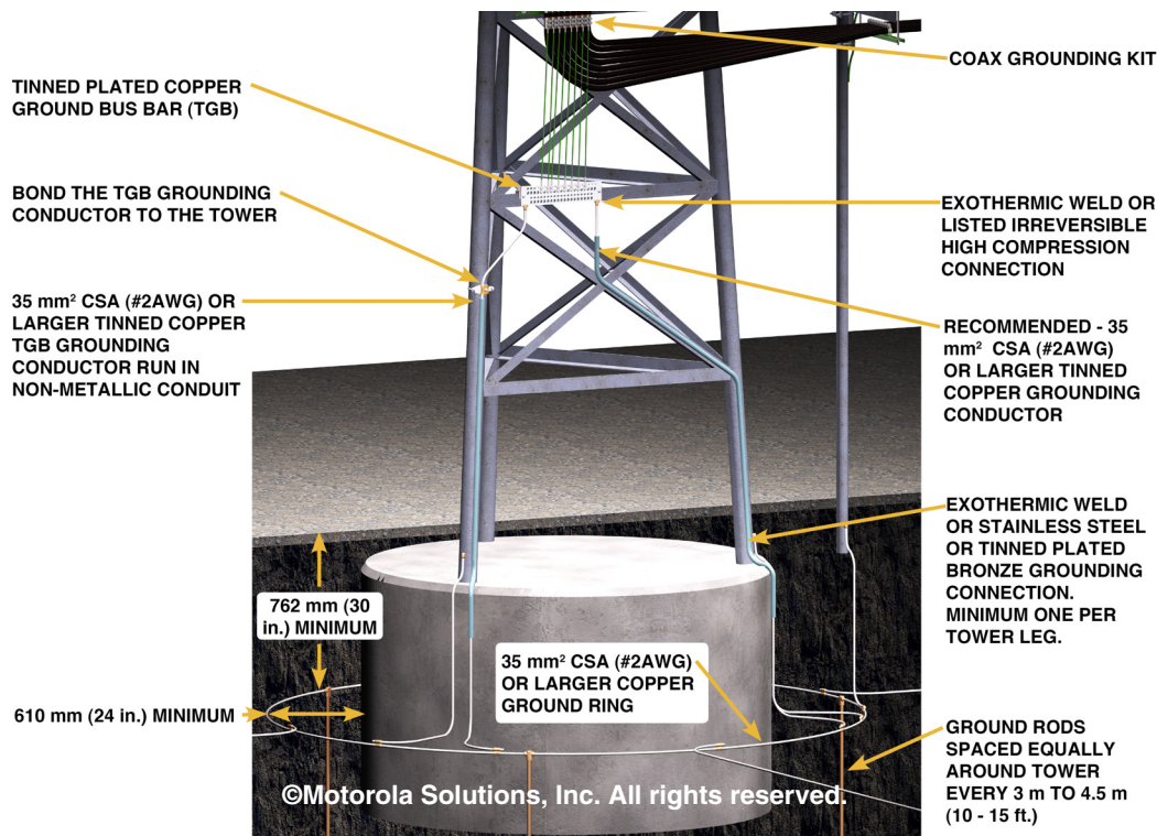
Figure 4-47 Bottom Tower Ground Bus Bar Configuration: Example 5
