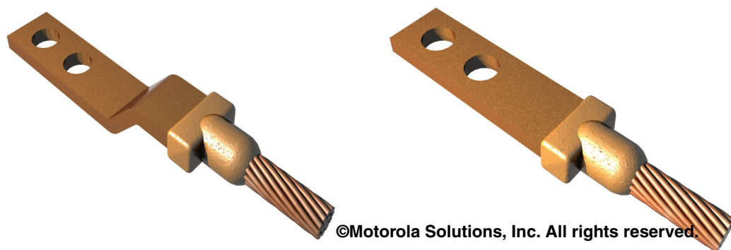
Figure 4-52 Lugs Exothermically Welded to Conductor
