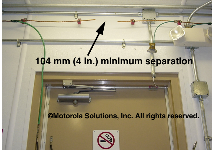
Figure 5-56 Example of Internal Perimeter Bonding Bus Conductors Separation - Opposite Primary Bonding Bar
