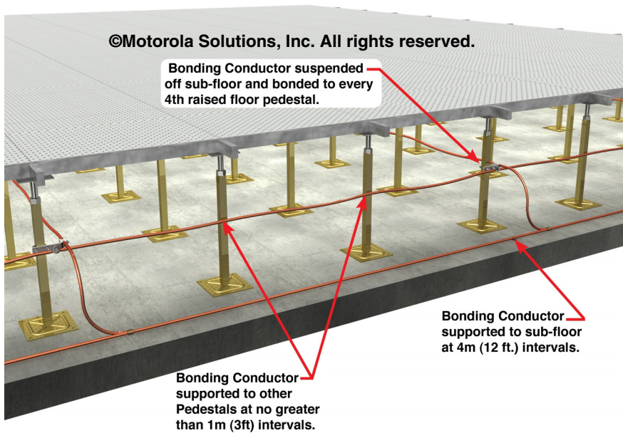
Figure 5-63 Example of Securing Grid Bonding Conductors Under Raised Flooring System
