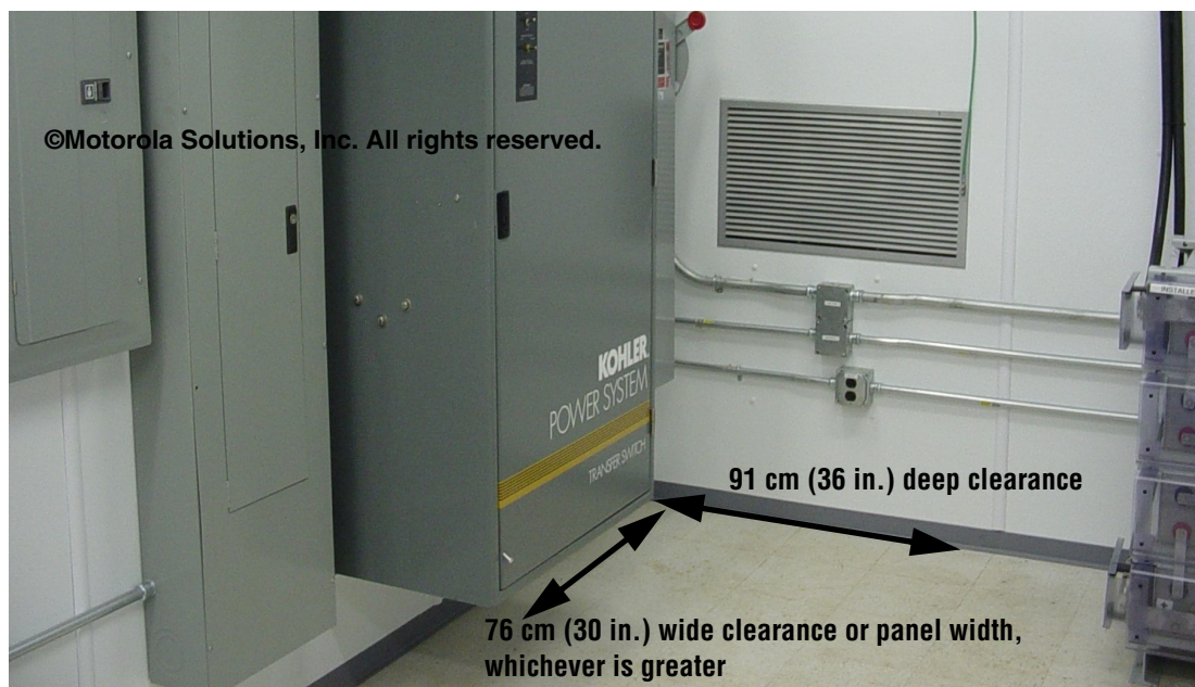
Figure 9-1 Example of Equipment Spacing
