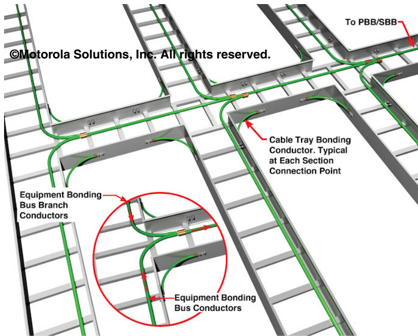
Figure 5-126 Example of Equipment Bonding Bus Conductors
