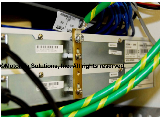
Figure 5-31 Example of Network-Equipment Bonding Bar
