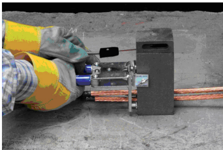
STEP 3: Attach ignition cord to the electronic igniter.
