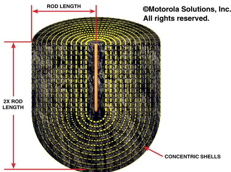
Figure 4-5 Ground Rod Sphere of Influence
