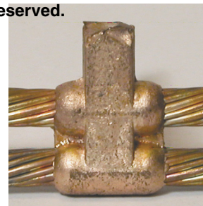
FINISHED CONNECTION
