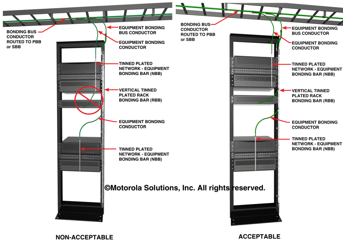
Figure 5-66 Daisy Chain Grounding Not Allowed
