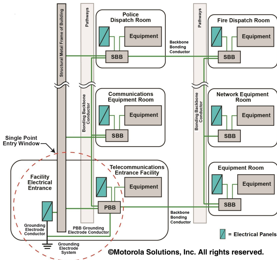
Figure 5-131 Example of Internal Bonding and Grounding System for Multi-Story Commercial Building
