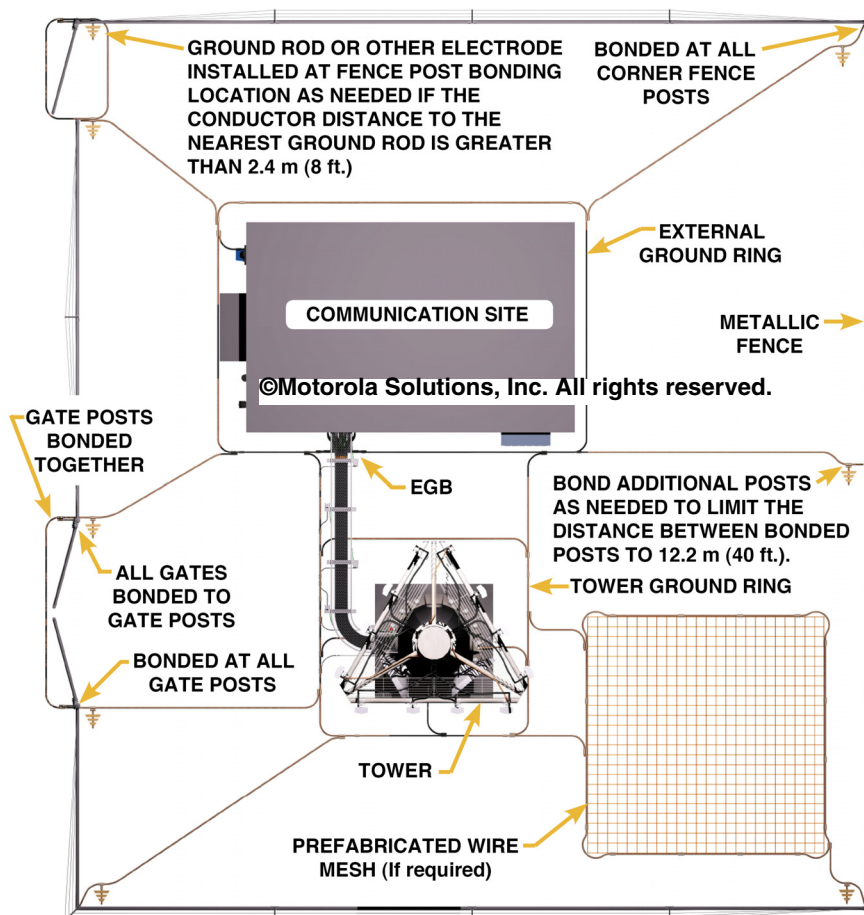
Figure 4-84 Example of Fence Grounding and Bonding
