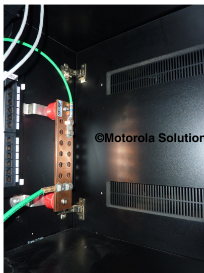
Figure 5-138 Example of Secondary Bonding Bar at Operator Position
