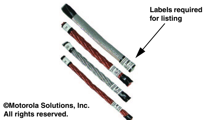
Figure 4-39 Lightning Protection System Grounding Conductor Examples
