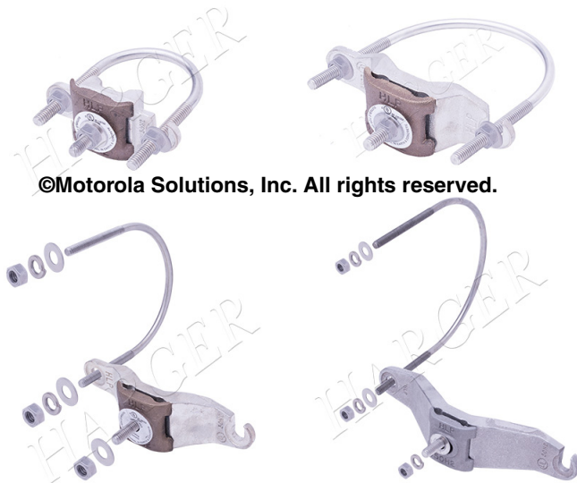
Figure 4-54 Examples of Pipe Bonding Clamps
