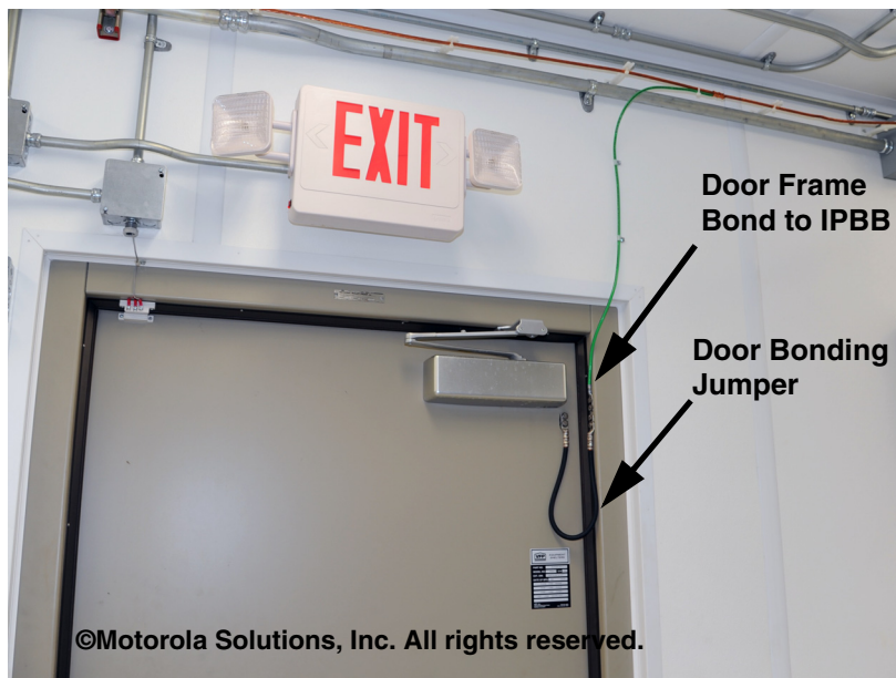
Figure 5-109 Example of Bonding Door Frame to Internal Perimeter Bonding Bus
