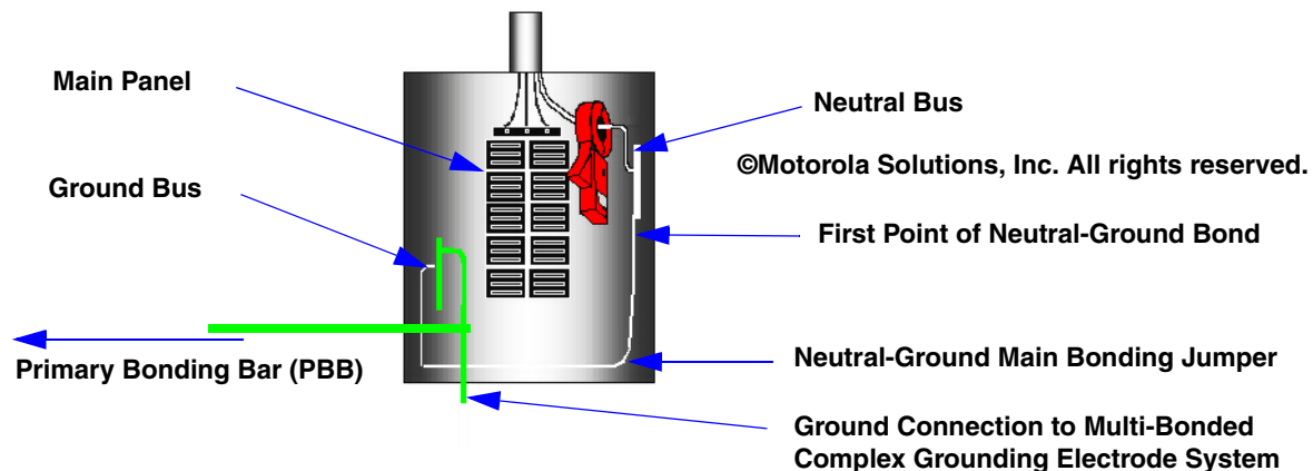
Figure D-17 Clamp-on Ohmmeter Placement For Multi-Bonded Complex Grounding Electrode System (Neutral-Ground Bond at Service Panel)
