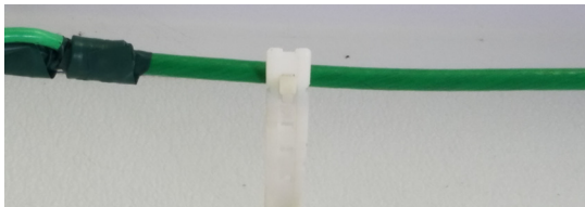
Figure 5-57 Example of Internal Perimeter Bonding Bus Mounting to Wall with Insulated Standoffs
