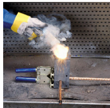
STEP 6: Wait 15 to 20 seconds for the reaction to complete, then open the mold and remove the welded connection. Remove slag from the mold before making the next connection.
