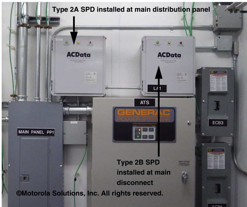
Figure 7-6 Example of AC SPD Installation at Typical Communications Site
