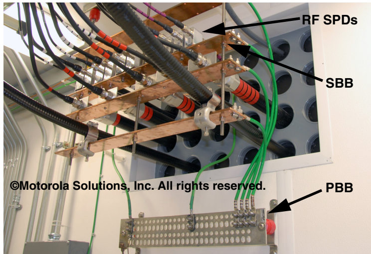
Figure 5-116 Example of RF Surge Protective Devices Bonding Directly to Secondary Bonding Bars
