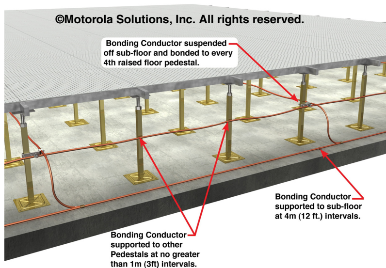
Figure 5-42 Securing Bonding Conductors Under Raised Flooring System
