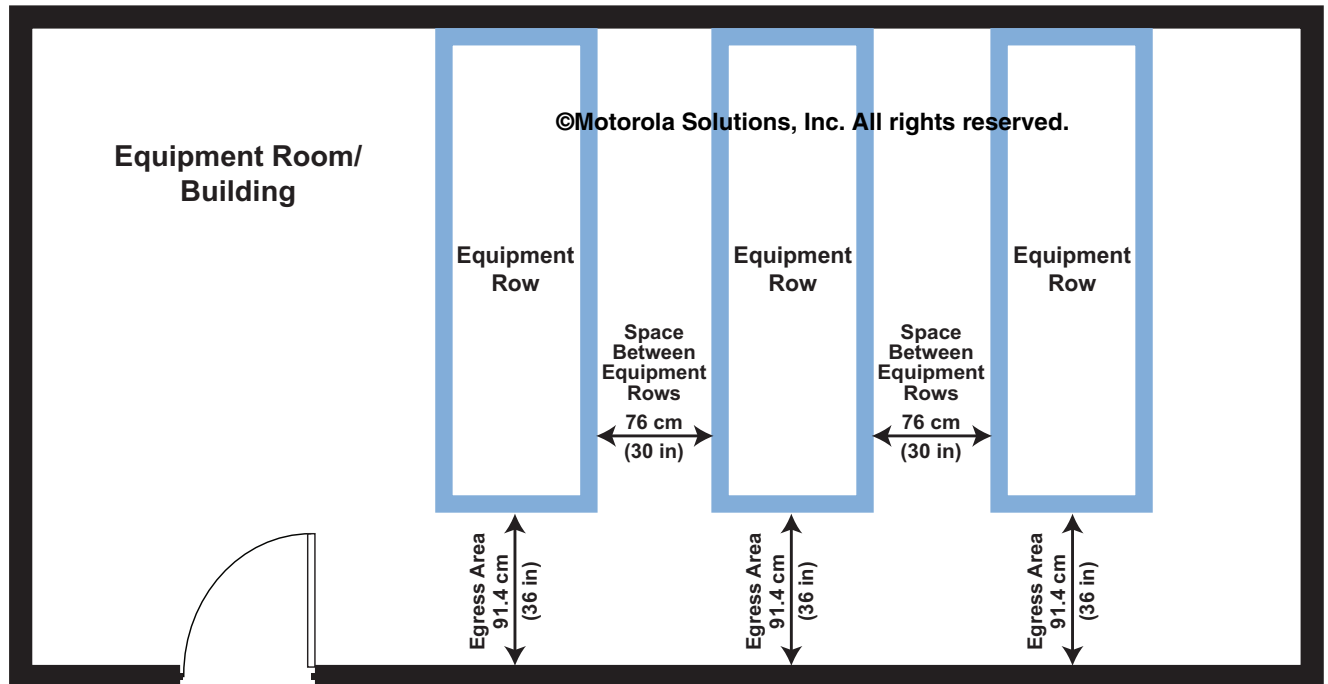
Figure 9-5 Example of Equipment Layout
