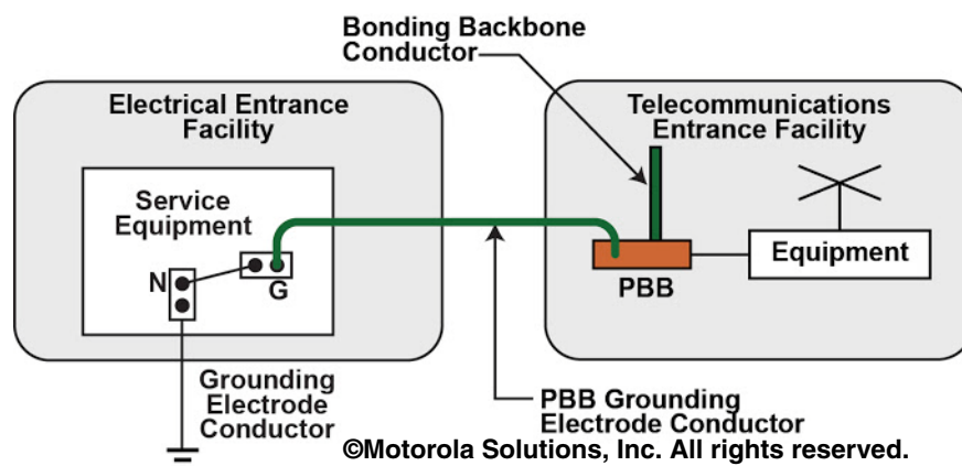
Figure 5-129 Example of Bonding to the Electrical Service (Power) Ground
