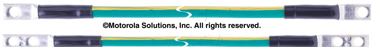
Figure 5-44 Examples of Premanufactured Bonding Jumpers
