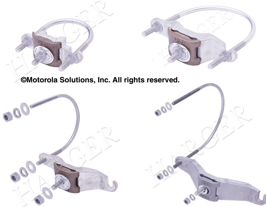
Figure 5-111 Examples of Pipe Bonding Clamps
