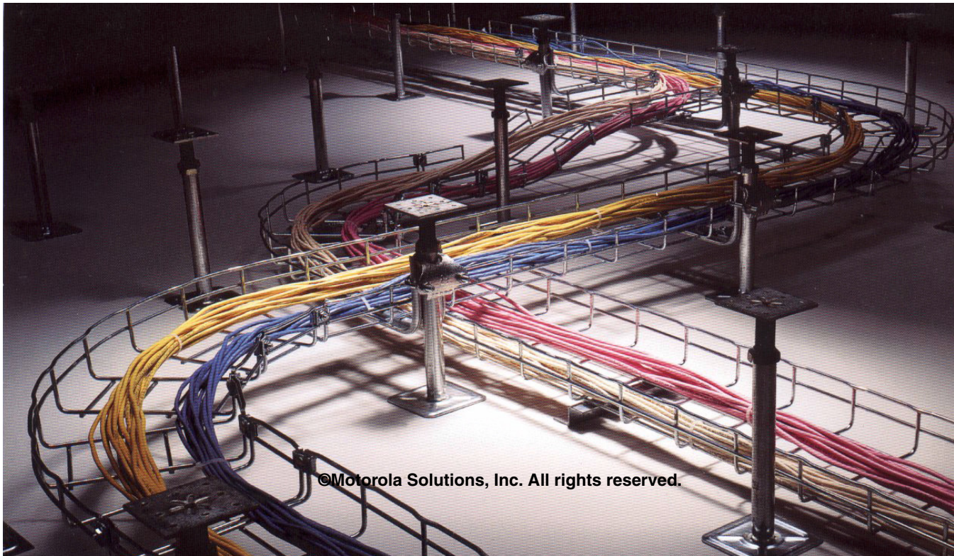
Figure 3-9 Typical Wire-Mesh Runway
