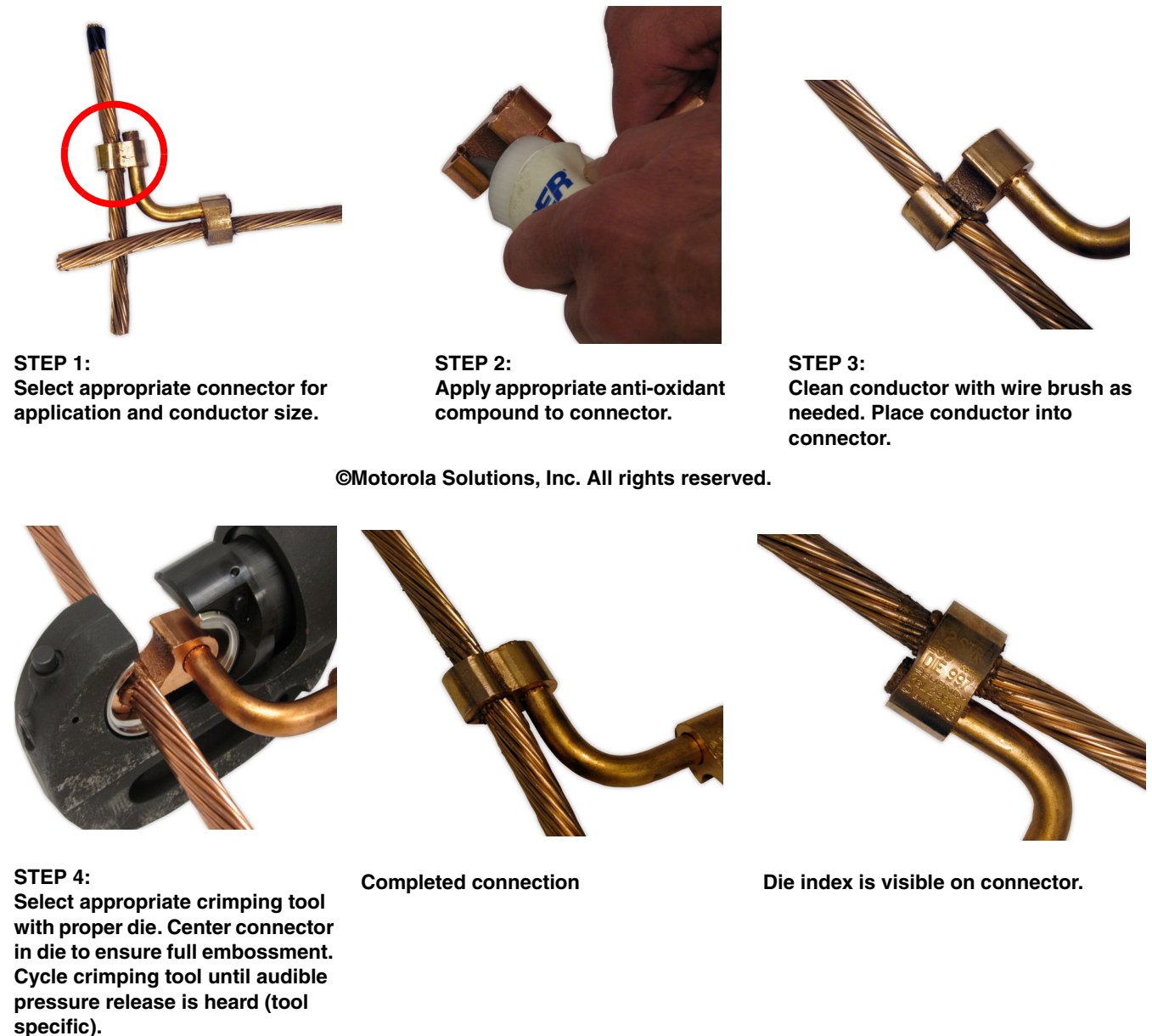
Figure 4-61 Typical High-Compression 90° Splice Connection Process
