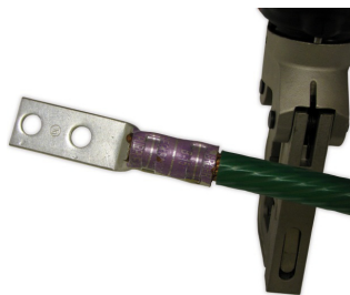
Figure 4-53 Irreversible Compression Connector and Typical Crimping Tool
