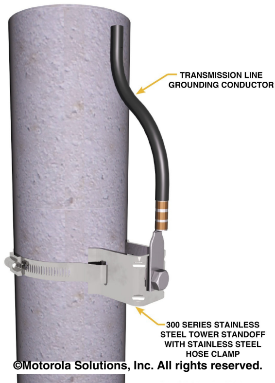
Figure 4-79 Grounding Transmission Line Top and Middle (Tubular Tower)
