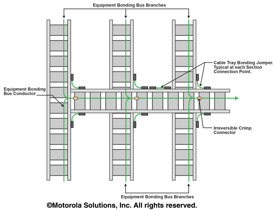
Figure 5-49 Example of Equipment Bonding Bus
