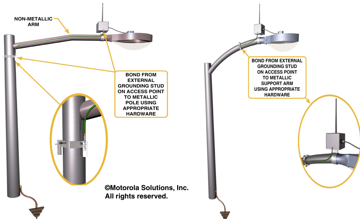
Figure 4-108 Grounding Access Point Mounted on Metal Pole
