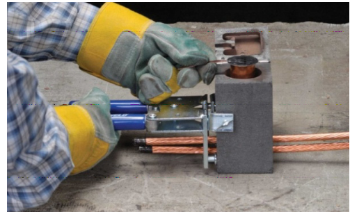
STEP 2: Close and lock handle clamp. Insert drop-in cartridge into mold.
