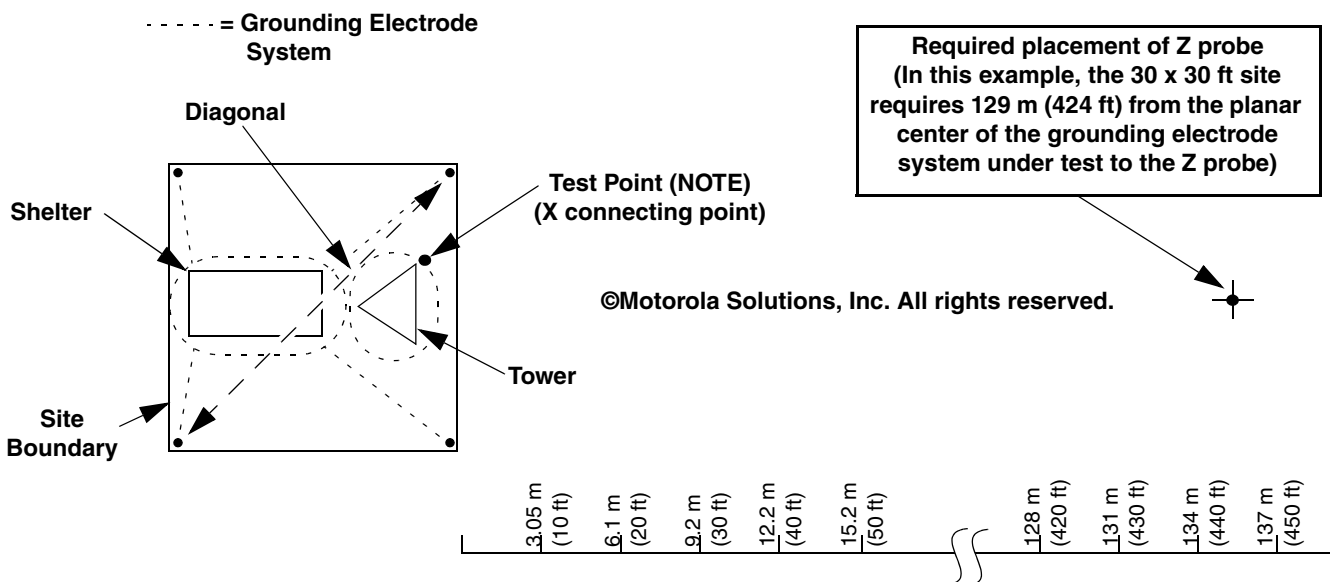
Figure D-4 Outer Reference Electrode (Z Probe) Placement for a Typical Site
