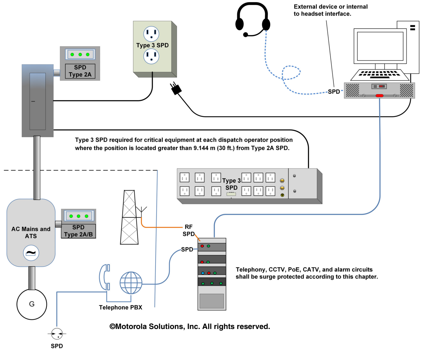
Figure 7-40 Example of Surge Protection Planning for Dispatch and Operations
