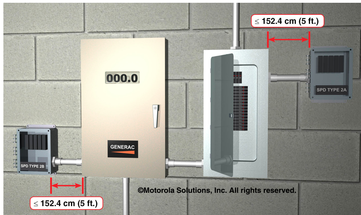
Figure 7-12 Example of SPD Conductor Length
