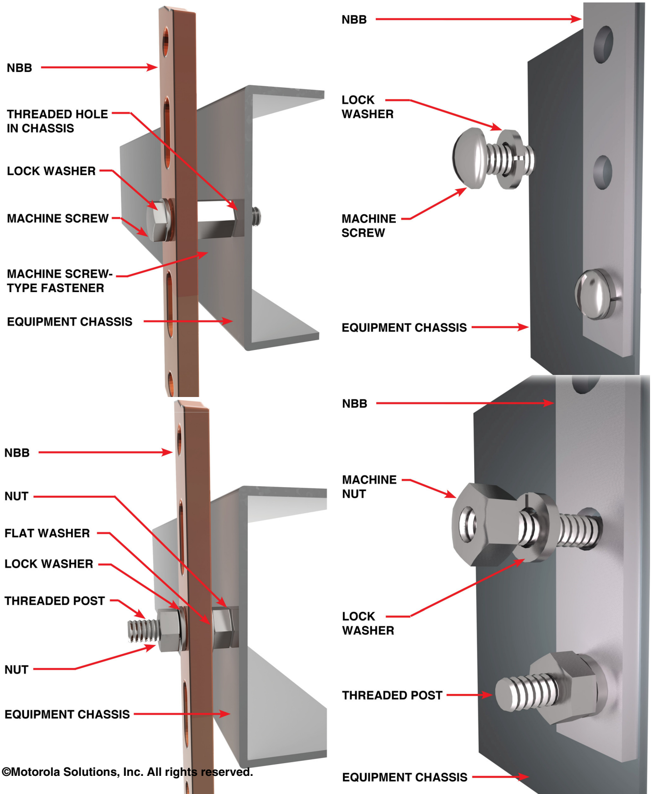
Figure 5-34 Examples of Bonding a Network-Equipment Bonding Bar to an Equipment Chassis with Lock Washers
