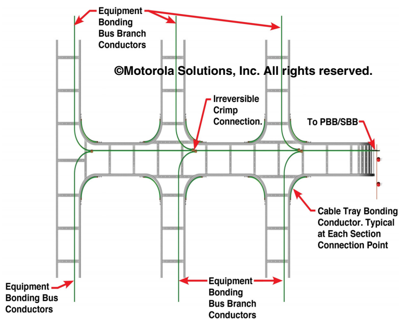
Figure 5-51 Example of Equipment Bonding Bus with Branch Conductors - Top View of Cable Trays
