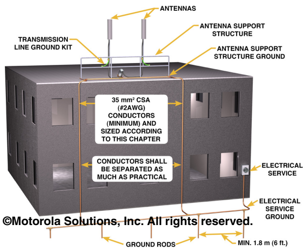
Figure 4-96 Roof Mounted Antenna Mast Grounding with Supplemental Grounding Electrode System
