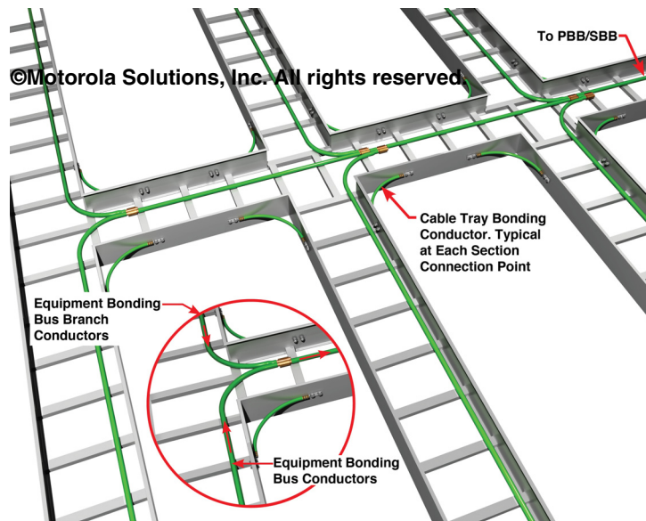
Figure 5-98 Example of Bonding Jumpers Installed on Cable Tray System (Top View)
