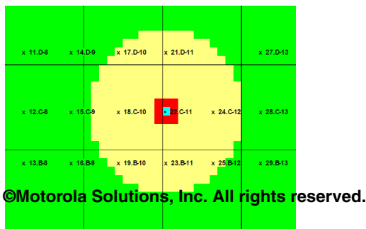
Figure A-9 Composite RF Fields with One Antenna Transmitting
