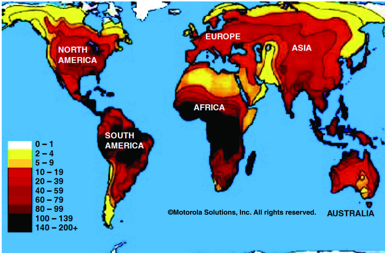
Figure 4-1 Lightning Activity, Thunderstorm Days Per Year
