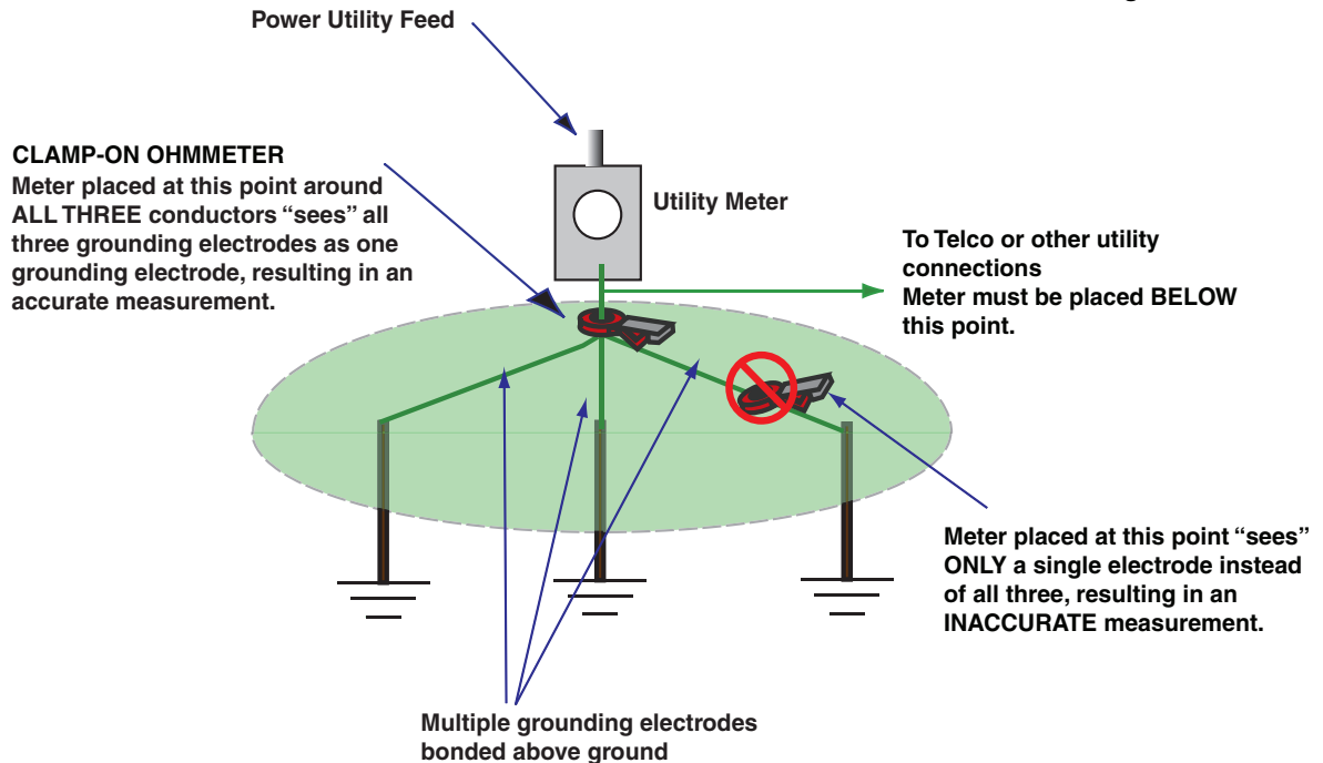
Figure D-15 Clamp-On Ohmmeter Placement
