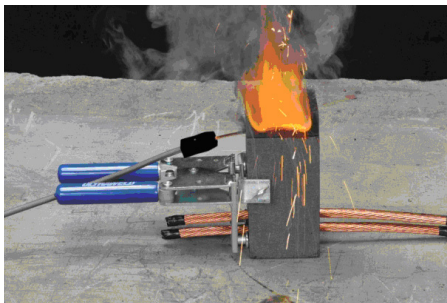
STEP 5: Reaction occurs. Wait 15-20 seconds, open mold and remove connection. Remove slag before making the next connection.
