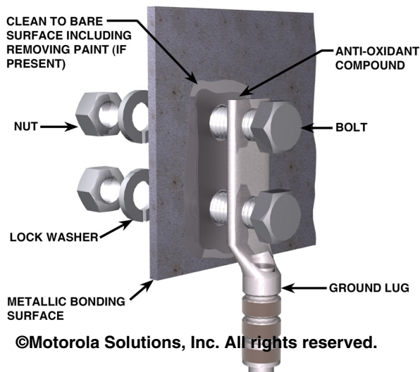
Figure 5-65 Proper Location of Washer When Connecting Ground Lug
